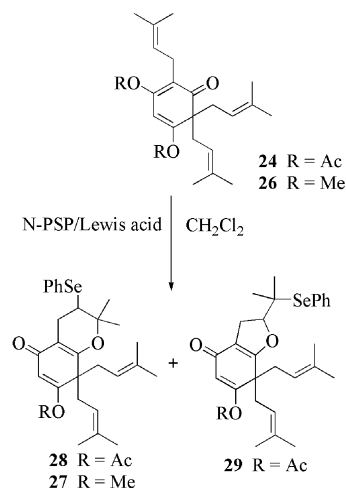
Scheme 8. N -PSP-induced cyclizations with 24 and 26 .
