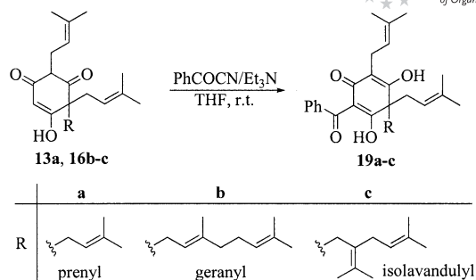
Scheme 6. C -Benzoylation of triprenylated phloroglucinols 13a , 16b and 16c .
