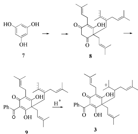
Scheme 2. Synthetic approach to PPAPs by triisoprenylated benzoylphloroglucinols.
