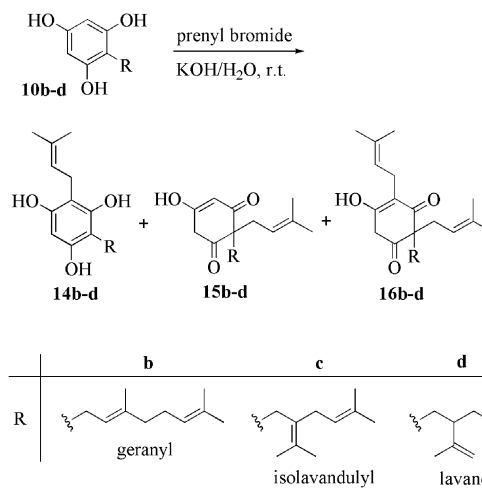
Scheme 4. Prenylation of monosubstituted phloroglucinols in water.
