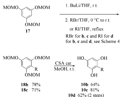
Scheme 5. Preparation of geranyl-, isolavandulyl- and lavandulyl-phloroglucinols.
