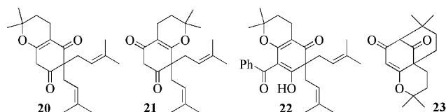
Figure 1. Products obtained by \text{SnCl}_4 -induced cyclization of 13a , 19a and 12a .
