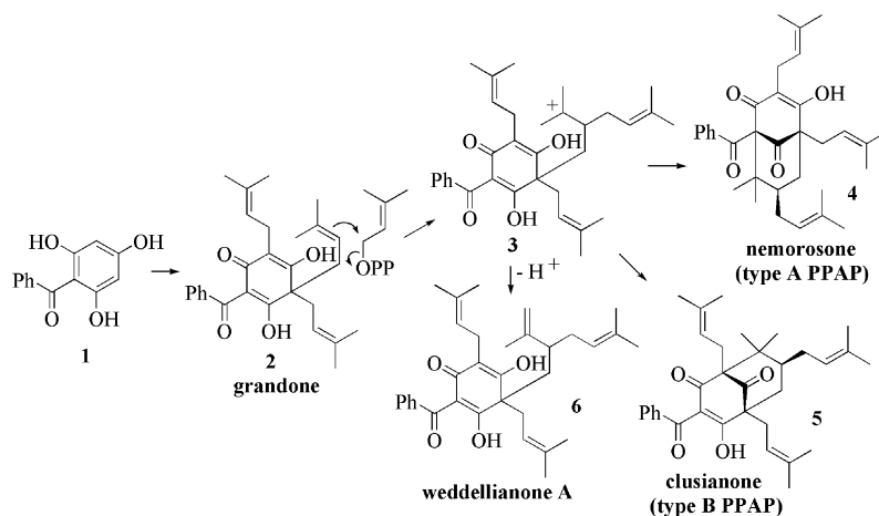
Scheme 1. Probable biosynthesis of PPAPs exemplified with benzoylphloroglucinol derivatives.
