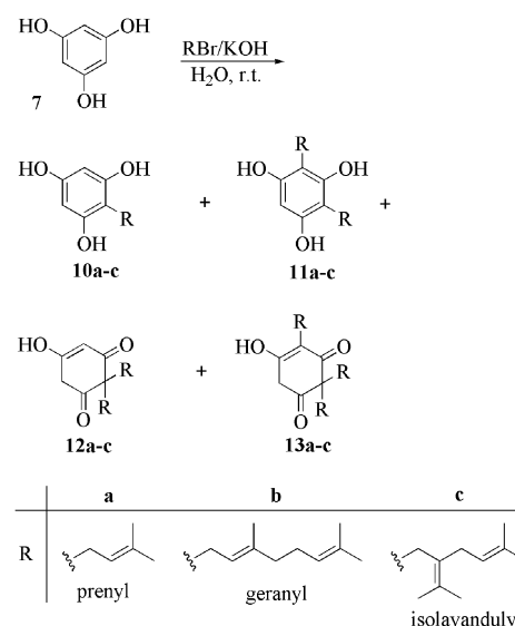
Scheme 3. Isoprenylation of phloroglucinol in water.
