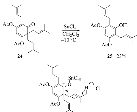
Scheme 7. Deprenylation of 24 with \text{SnCl}_4 .
